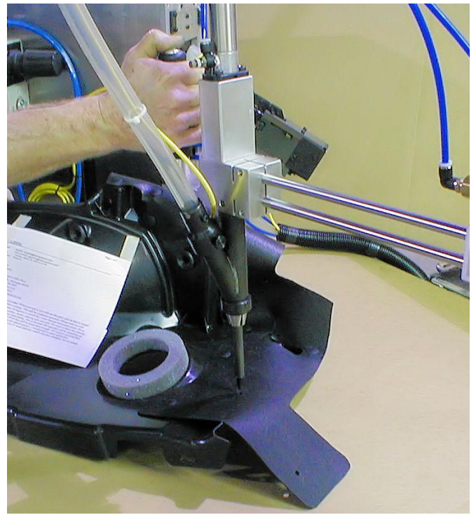
Inserting plastic push pins
