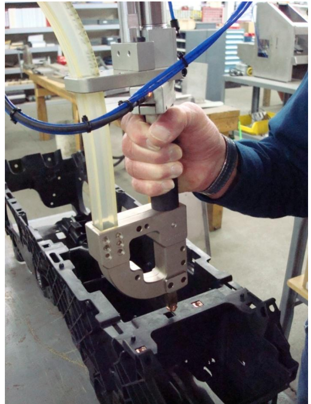
Placing M4 panel nuts into a center console
